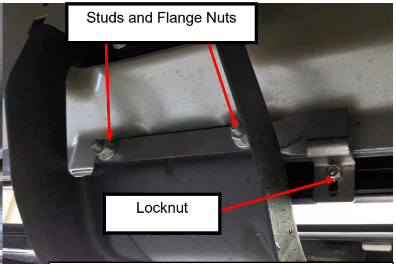
Figure 4b. Fastening Extrusion to Vehicle
