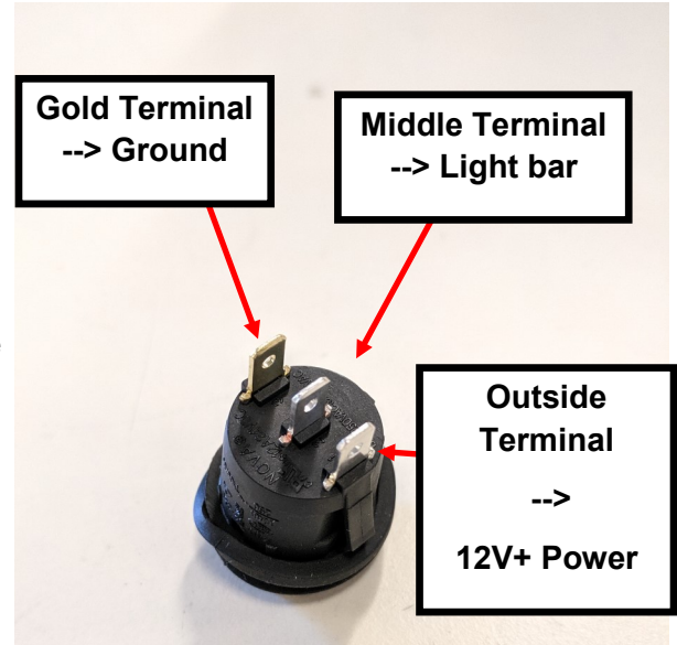
Figure 5. Switch terminal identification
